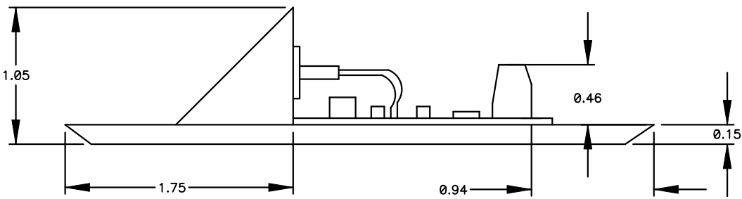
SM1-TR SIDE-LEFT
