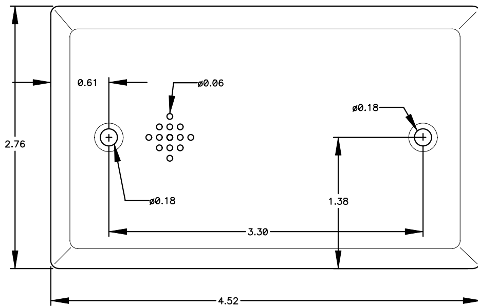
SM1-TR FRONT
