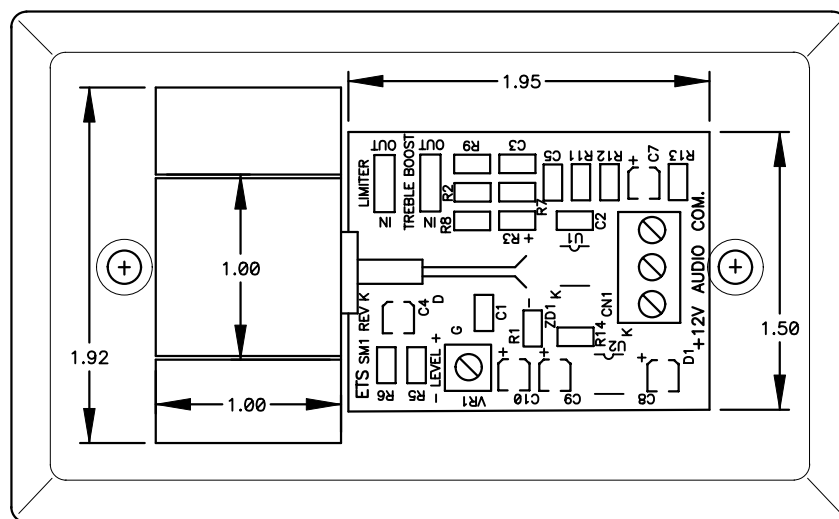
SM1-TR REAR
